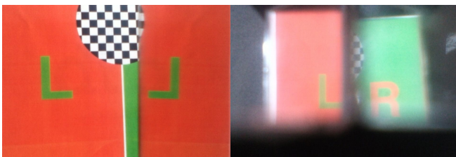
Figure 4: Results of the single lens viewers, on the left the solution with only one mirror, on the right the solution with 4 prism,
